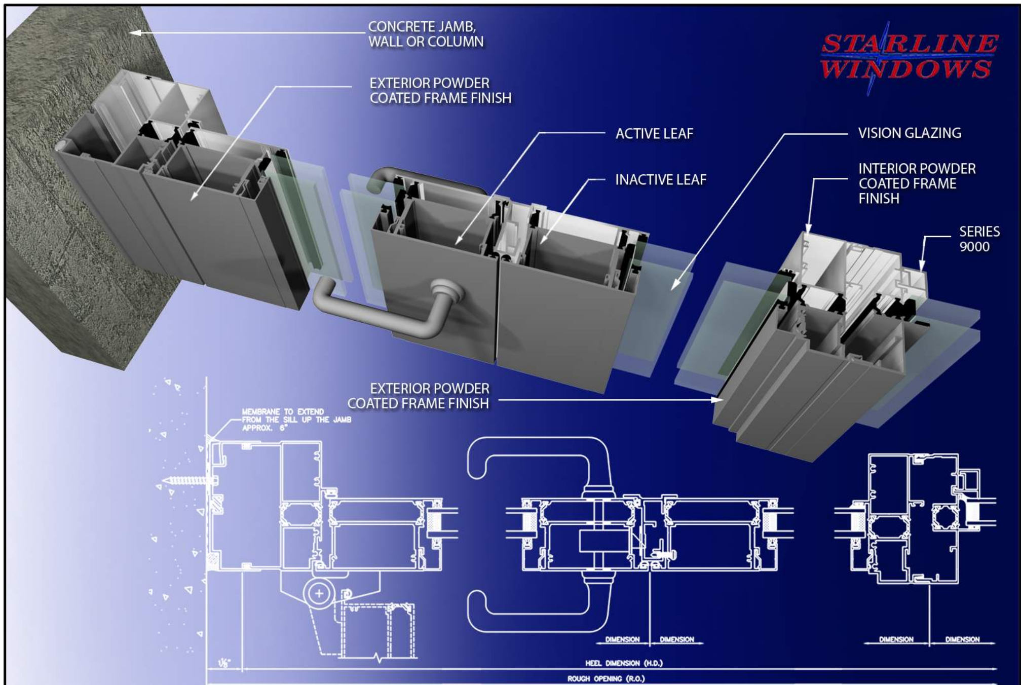
SERIES 9502 - FRENCH DOOR - SEISMIC JAMB, ASTRAGAL & 180 DEGREE COUPLER
