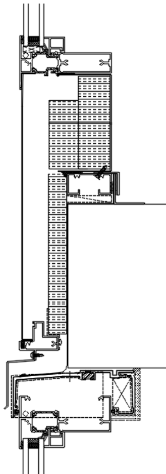
EXTERIOR: ALUMINUM PANEL INTERIOR: ALUMINUM BACK PAN
