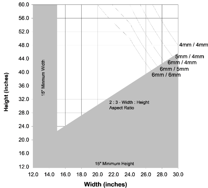
Recommended Maximum Sizes of 9100R Series Casement with Restrictor
