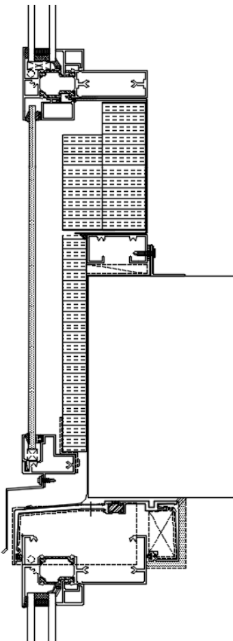
EXTERIOR: SPANDREL GLASS INTERIOR: ALUMINUM BACK PAN
