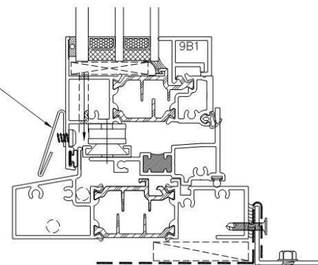
Operable Vent — Triple Glazed
