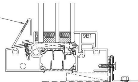
Fixed Window — Triple Glazed
